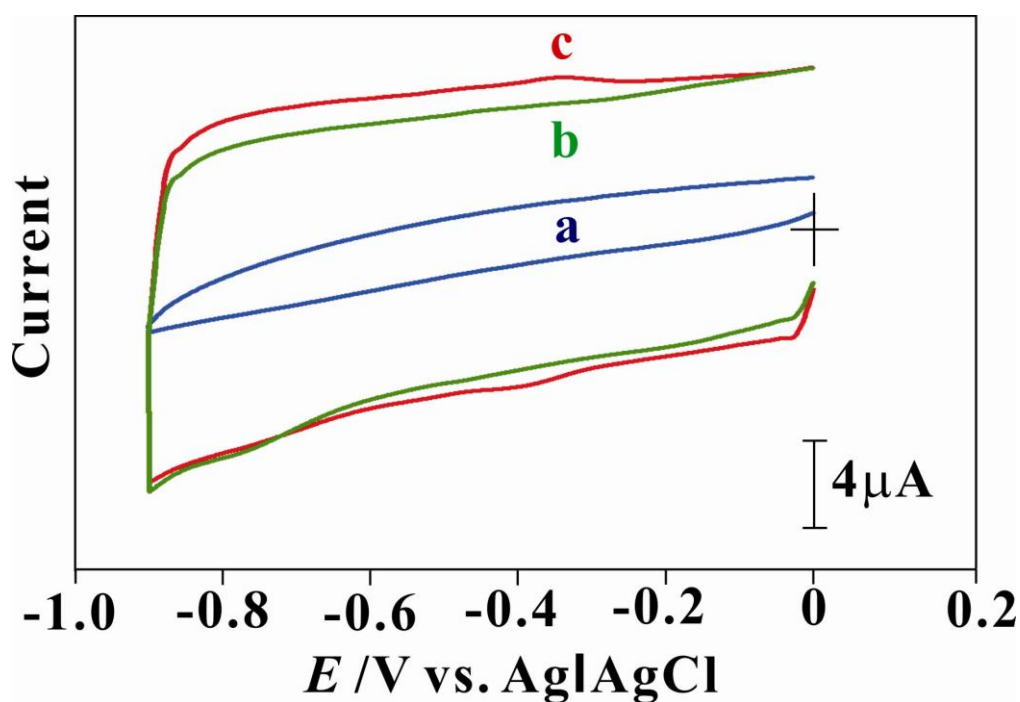
Figure 1. Cyclic voltammograms of (a) bare GCE, (b) MWCNTs/GCE, and (c) ChOx/MWCNTs/GCE examined in 0.1 M PBS (pH 7.0), scan rate = 100 mV s -1 .
