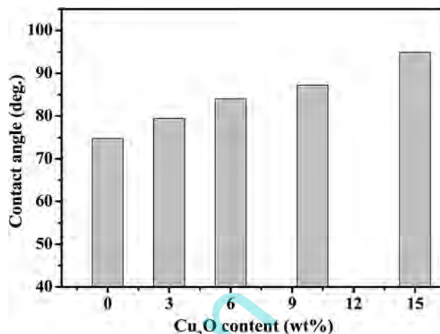
Fig. 9 Effect of Cu 2 O content on water contact angle of the membrane.
